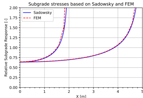
Figure 2. Vertical subgrade stresses estimated by FEM and Sadowsky's equation for two foundation widths; 4 m and 10 m.
