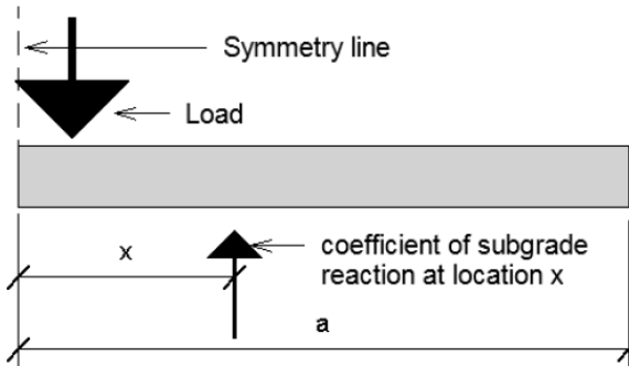
Figure 1. Cross section of a strip foundation
