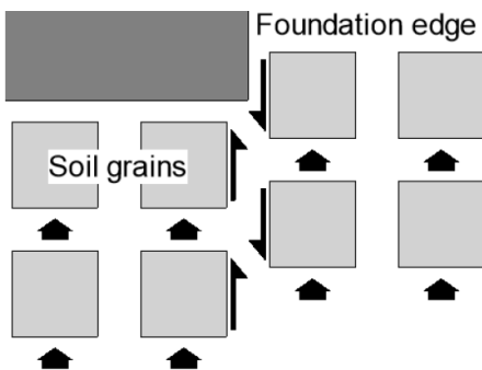
Figure 4. Shearing stress contribution along foundation edge
